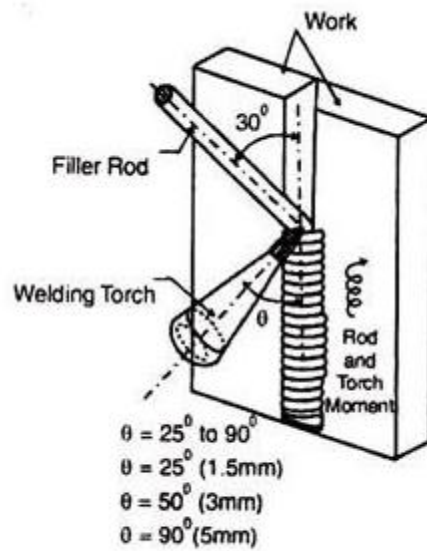
Fig 7.13. Vertical Welding.
